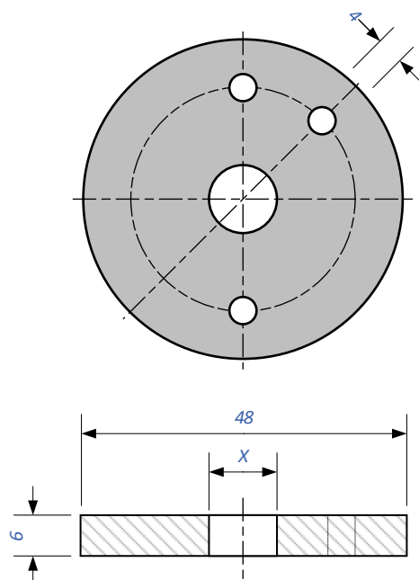
Feedpoint spreader
