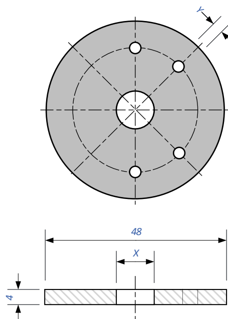
Reflector spreader
